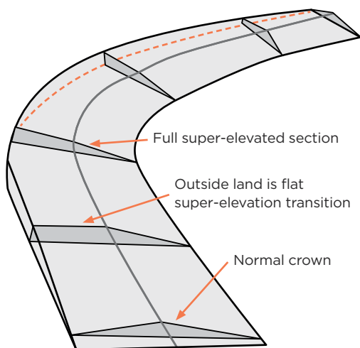
FIGURE 22: Super-elevated bends
