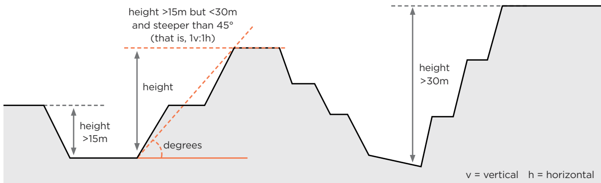
FIGURE 7: 'Stronger rock' guidance
