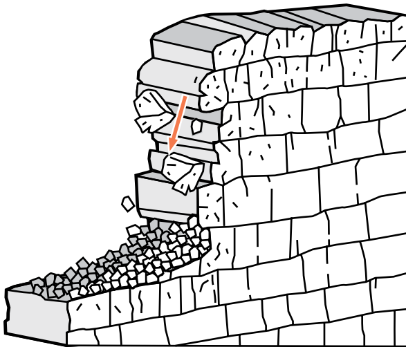
FIGURE 12: Ravelling failure
